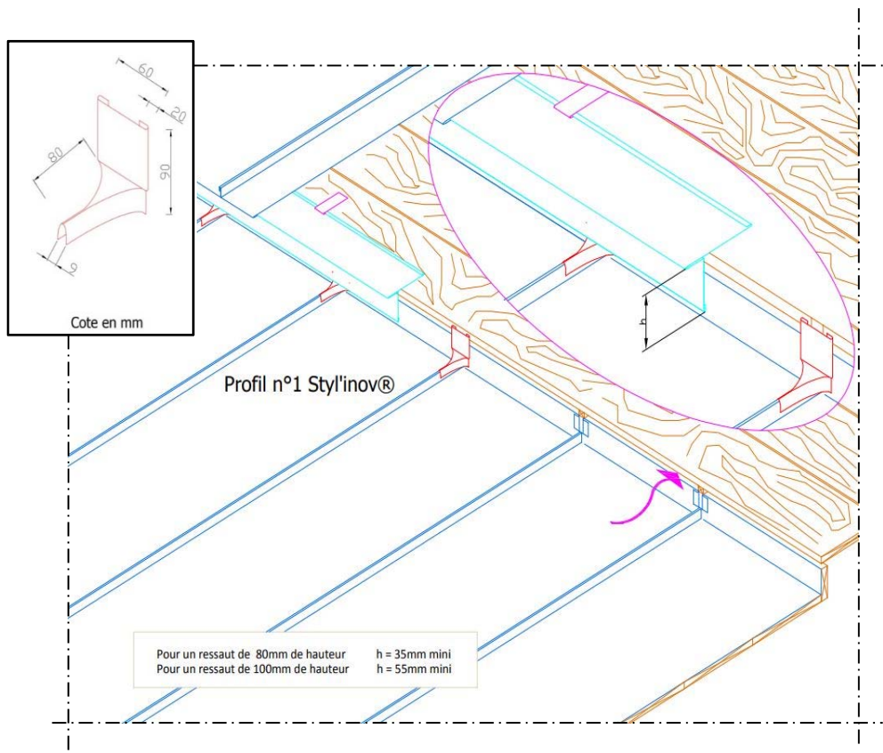
Figure 19 – Ressaut
