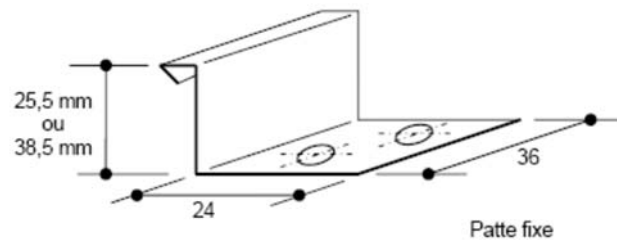
Figure 2a – Patte fixe
