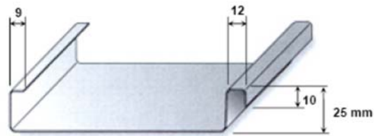
Figure 1a – Profil joint 25 mm
