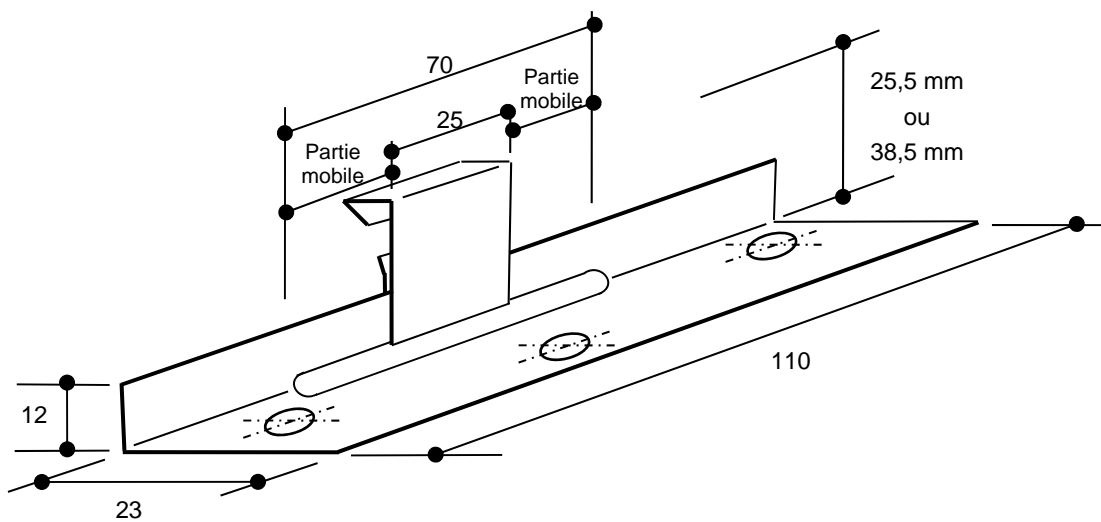
Figure 2b – Patte coulissante
