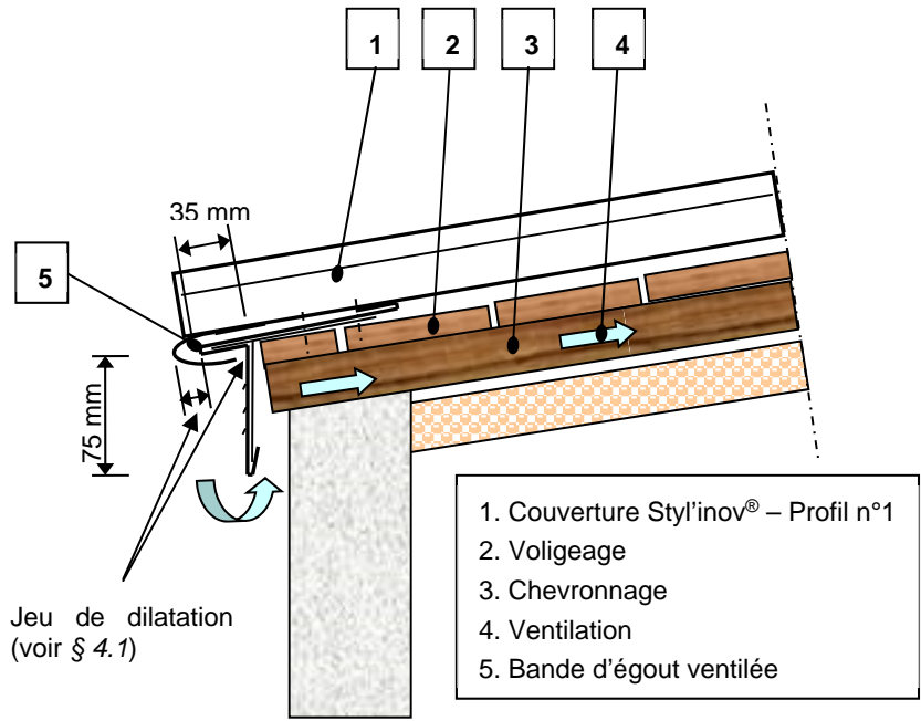
Figure 11 – Égout
