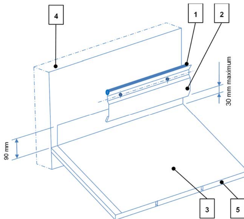
Figure 15 – Noue encaissée
