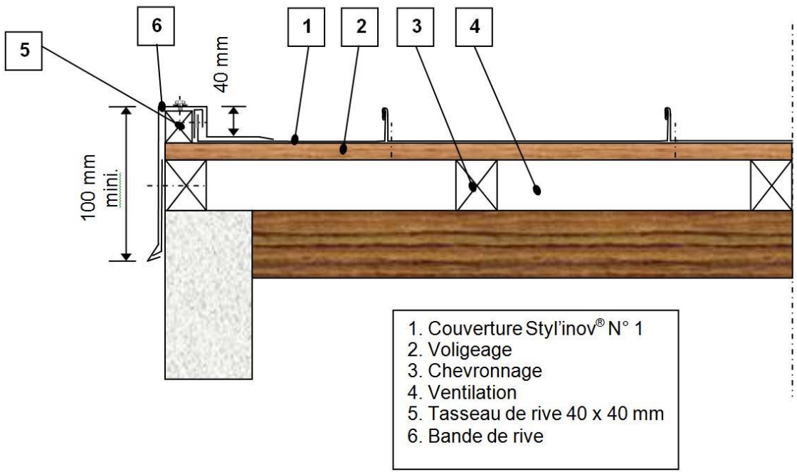
Figure 12 - Rive
