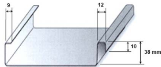
Figure 1b – Profil joint 28 mm
